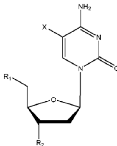
Formula (IIa)
