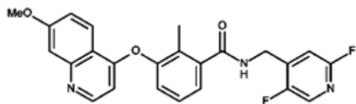
Formula (CXCII)
