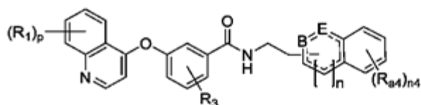
Formula (XVIa-1)
