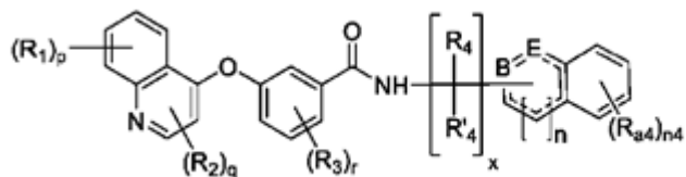
Formula (VIIIa)
