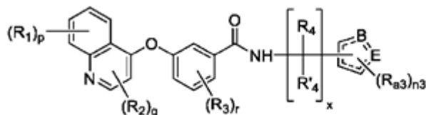
Formula (VIIa)
