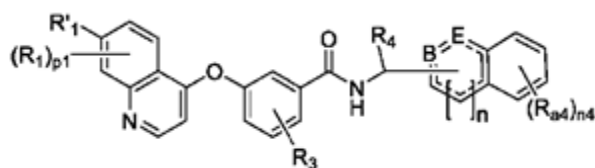
Formula (VIIIa-a1)
