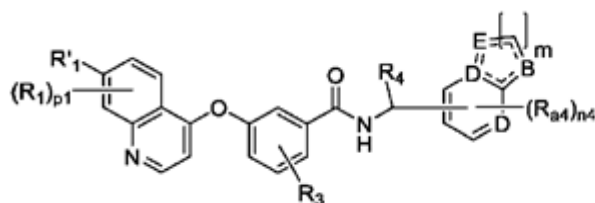
Formula (IXa-a1)
