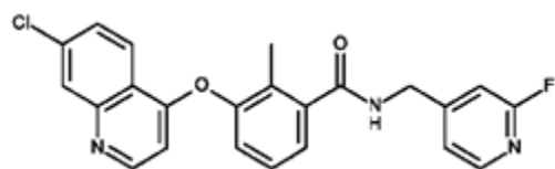
Formula (CLXXXVI)
