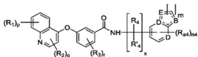
Formula (IXa)
