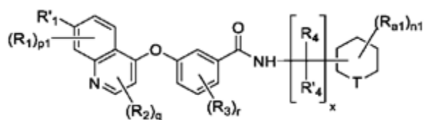
Formula (IIa-a)
