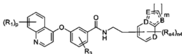
Formula (XVIIa-1)
