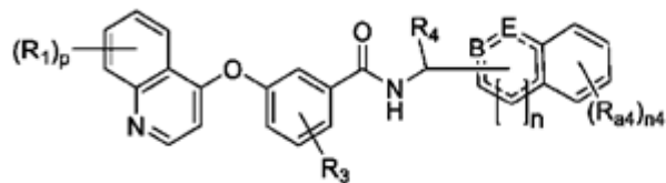
Formula (VIIIa-1)
