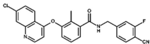
Formula (CLXXXVIII)
