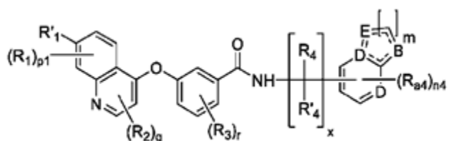
Formula (IXa-a)
